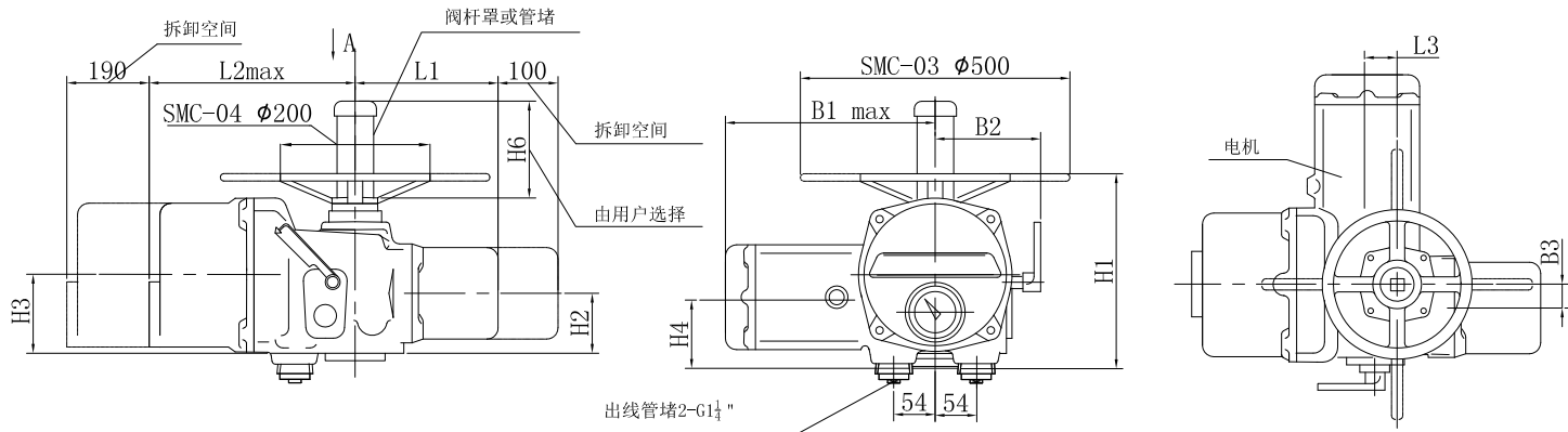
SMC-04~03基本型外形尺寸
